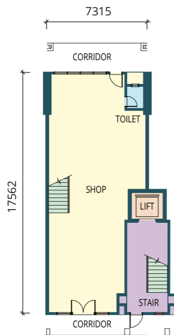
GROUND FLOOR Floor Area: 1,228 sq.ft. Total Area: 1,881 sq.ft.
