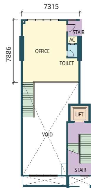
MEZZANINE FLOOR Floor Area: 652 sq.ft.
