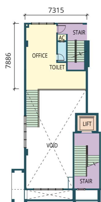
MEZZANINE FLOOR Floor Area: 527 Sqft
