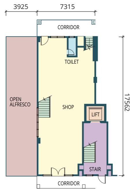
GROUND FLOOR Floor Area: 1,210 Sqft ACCESSORY PARCEL (OPEN ALFRESCO) : 742 SQFT Total Area: 2,479 sq.ft.
