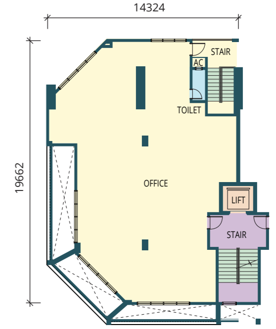
SECOND FLOOR Total Area: 2,240 sq.ft.
