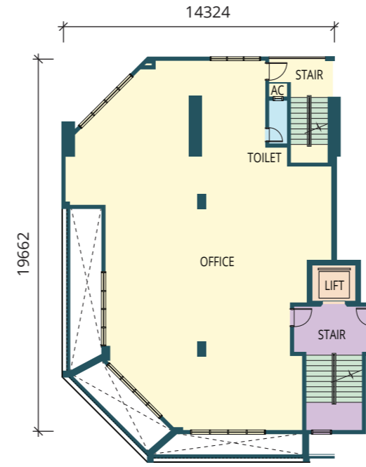
FIRST FLOOR Total Area: 2,240 sq.ft.
